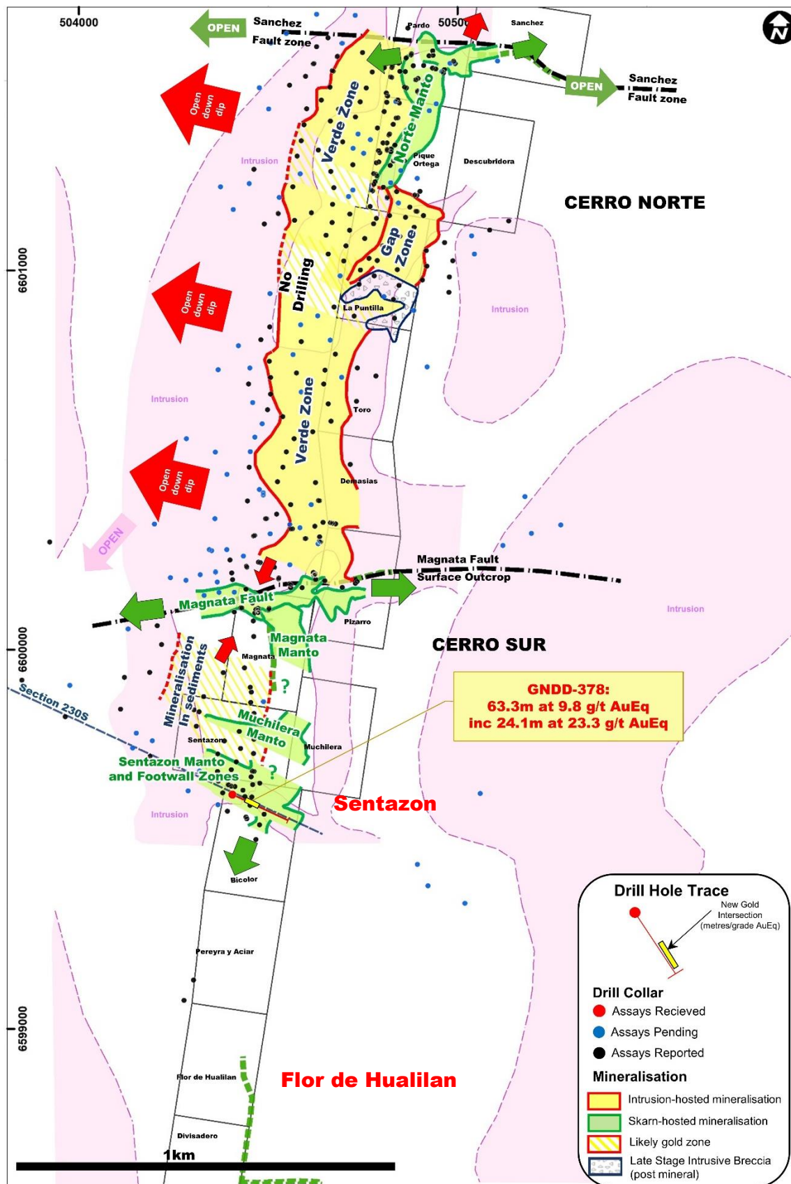
Figure 2 - Plan View Hualilan Project showing Sentazon Location
